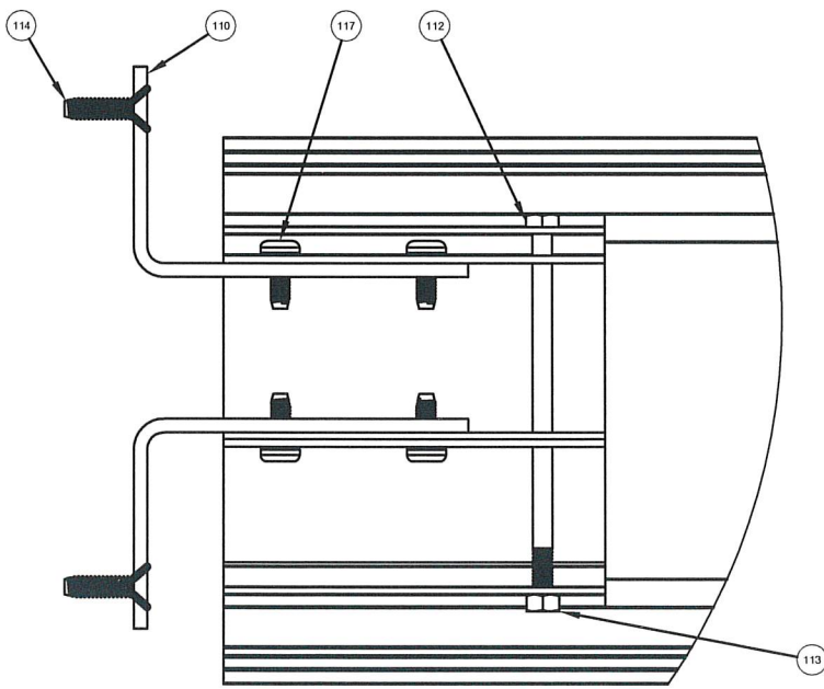
Section F-F True Divided 4" Muntin
