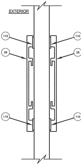
Section E-E 2" Surface Applied Muntin
