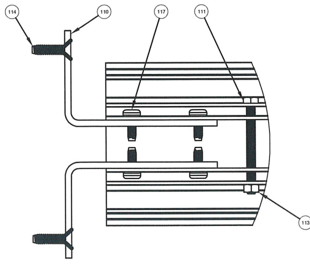
Section G-G True Divided 2" Muntin
