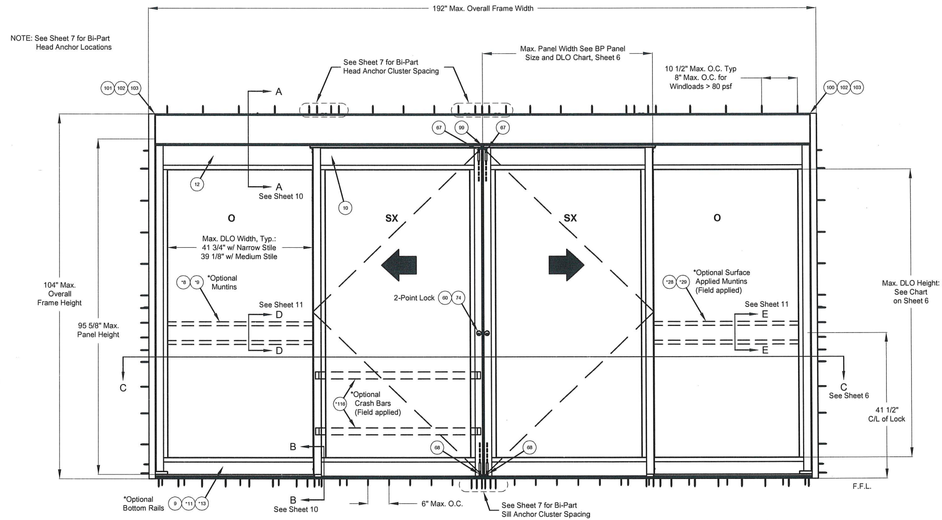
BP FSL (4 PANELS, BI-PART FIXED SIDELITE)
